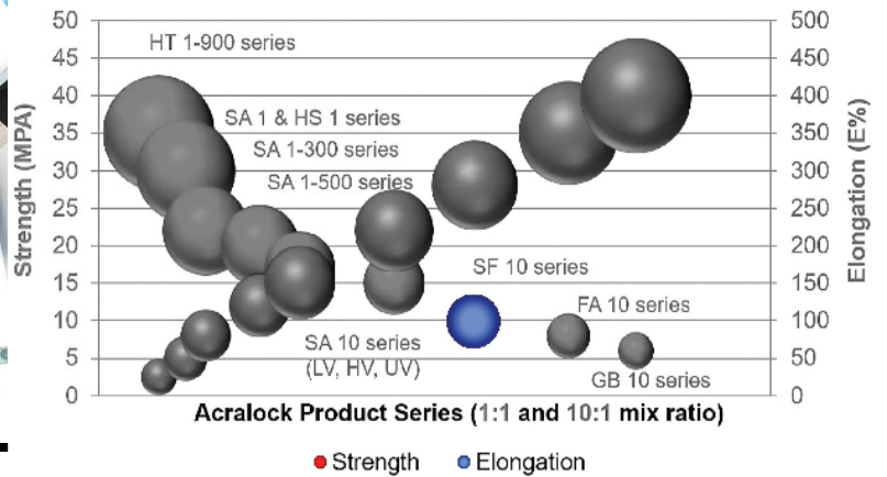
Basic Mechanical Properties of EBS Acralock Structural MMA Adhesive Product Range
