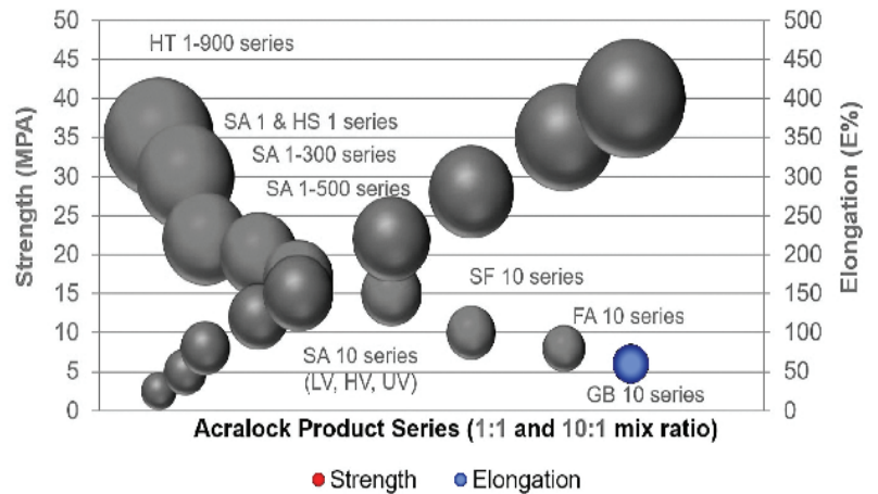
Basic Mechanical Properties of EBS Acralock Structural MMA Adhesive Product Range
